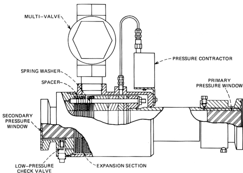
Fig. 6—Multifunction waveguide.
